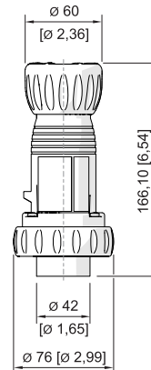
8573/12-... SolConeX extra-low voltage plug
